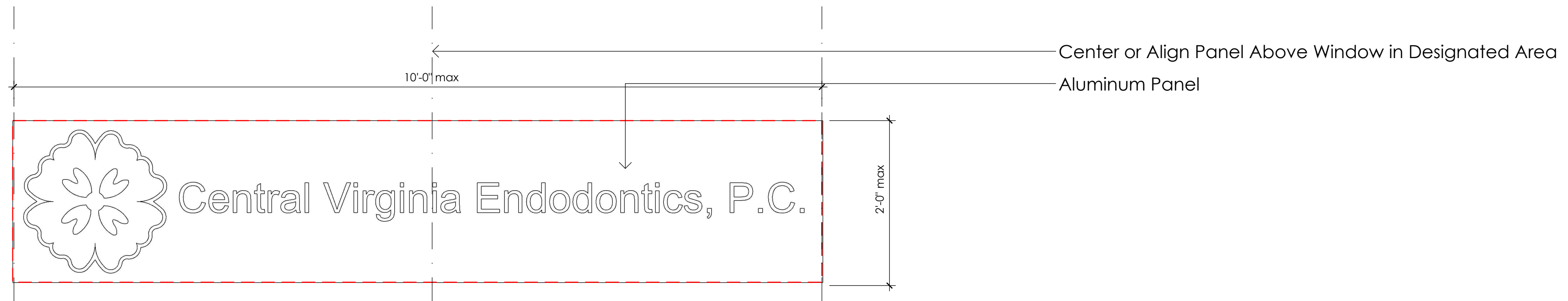
2 WALL SIGN FRONT ELEVATION CSP.6 1" = 1'-0"
